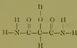
\text{C}_3\text{H}_2\text{H}_3(\text{NH}_2)_2 Tartronylamid.
